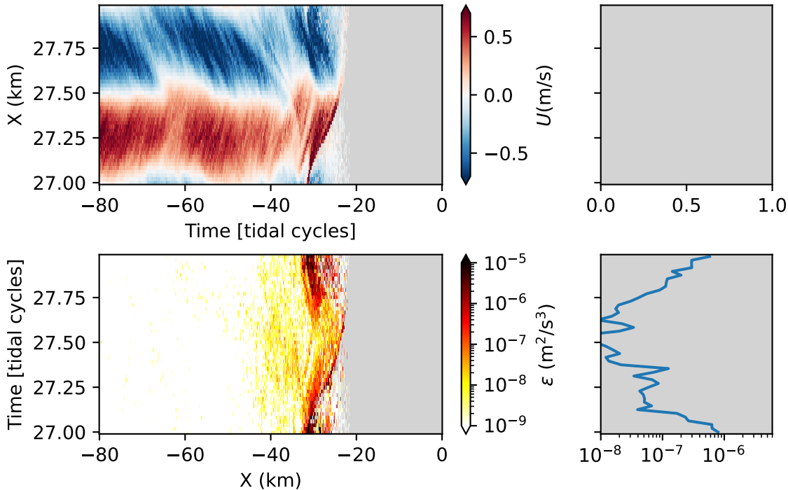
Slope2D091: Hovmoller along [25.6] isopycnal
