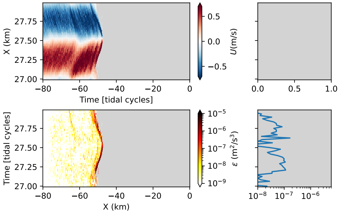
Slope2D096: Hovmoller along [25.6] isopycnal
