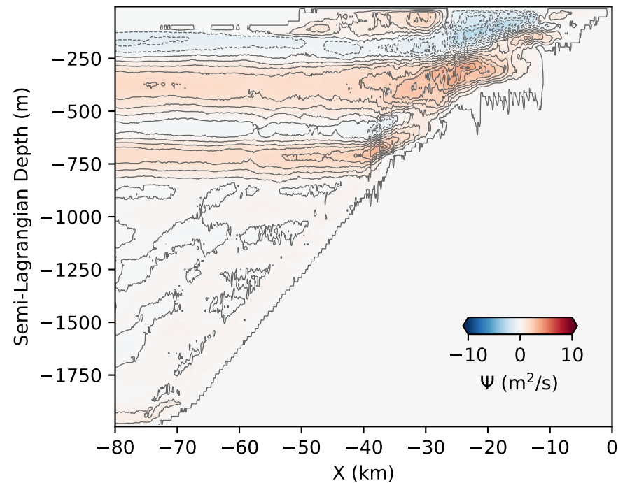
a) Sub-critical slope, u_0=0.6 m/s
