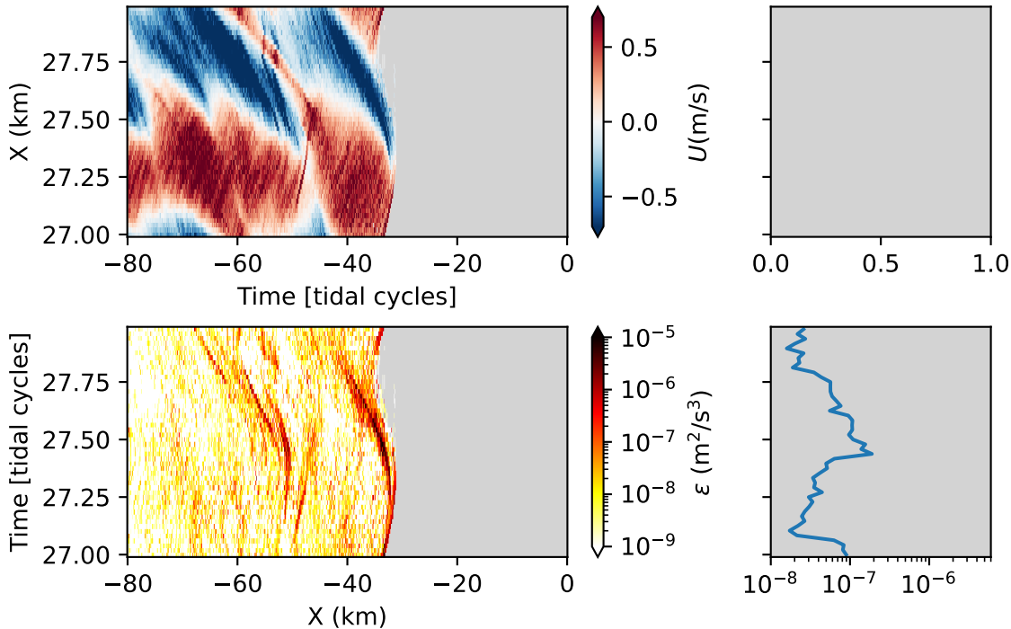
Slope2D097: Hovmoller along [25.6] isopycnal
