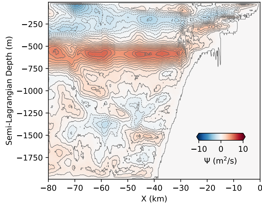
a) Super-critical, u_0=0.6 m/s
