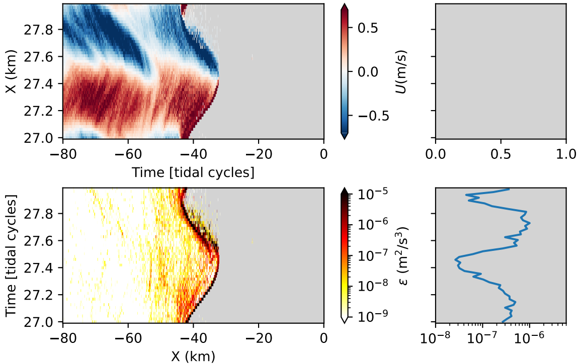
Slope2D098: Hovmoller along [25.6] isopycnal
