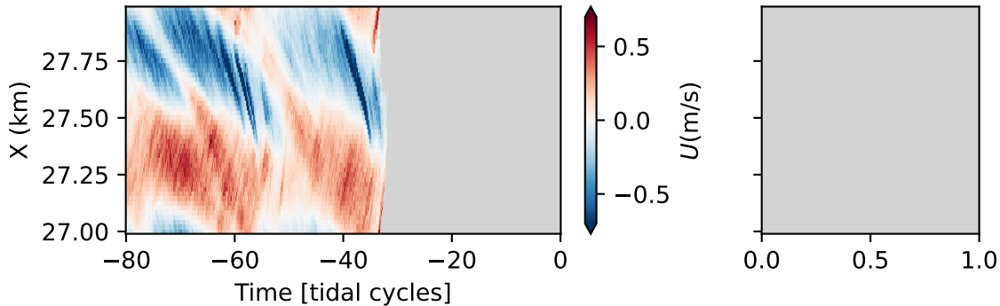
Slope2D099: Hovmoller along [25.6] isopycnal
