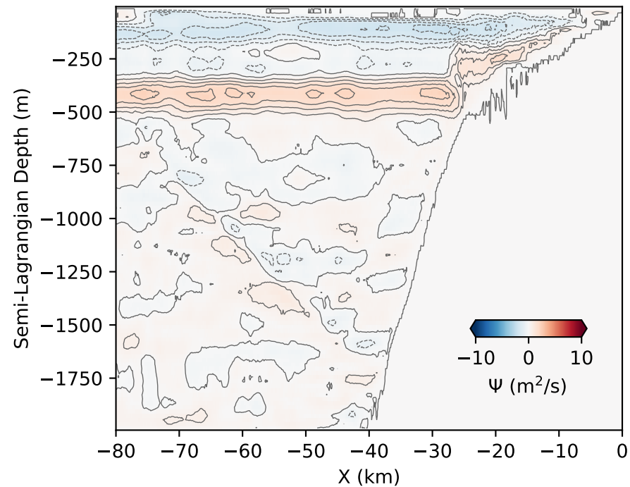
a) Super-critical slope, u_0=0.3 m/s
