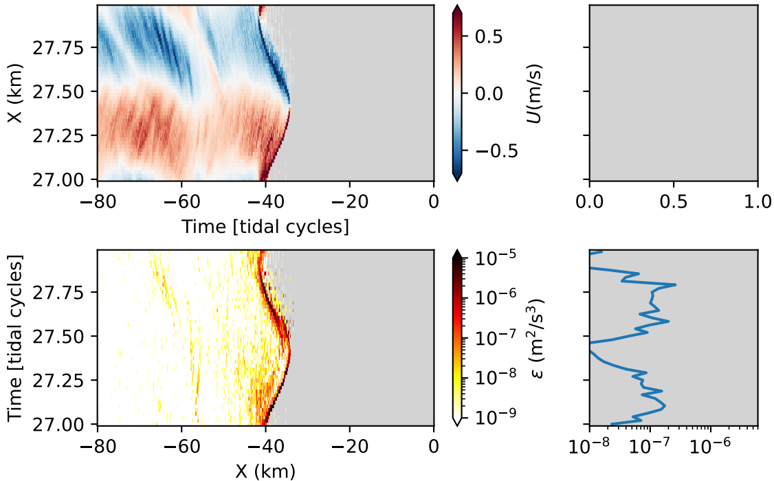
Slope2D100: Hovmoller along [25.6] isopycnal
