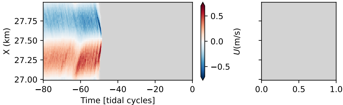
Slope2D101: Hovmoller along [25.6] isopycnal
