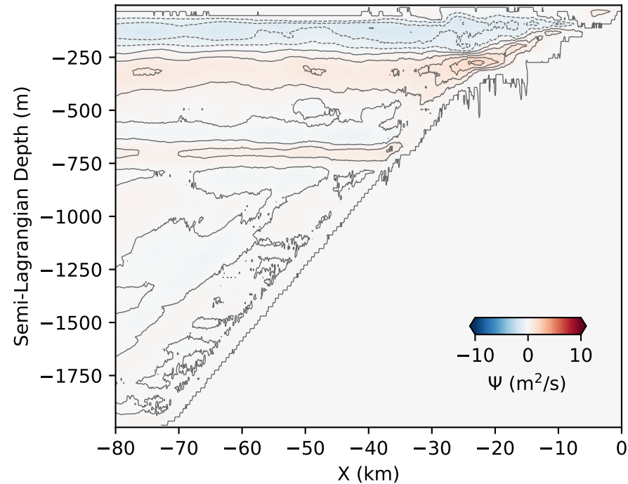
a) Sub-critical slope, u_0=0.3 m/s
