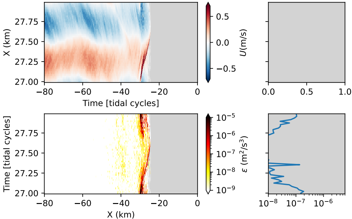
Slope2D102: Hovmoller along [25.6] isopycnal
