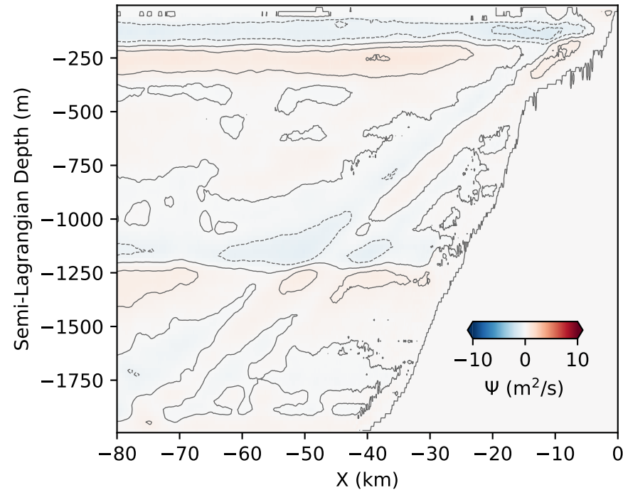
a) Multiple slopes, u_0=0.3 m/s
