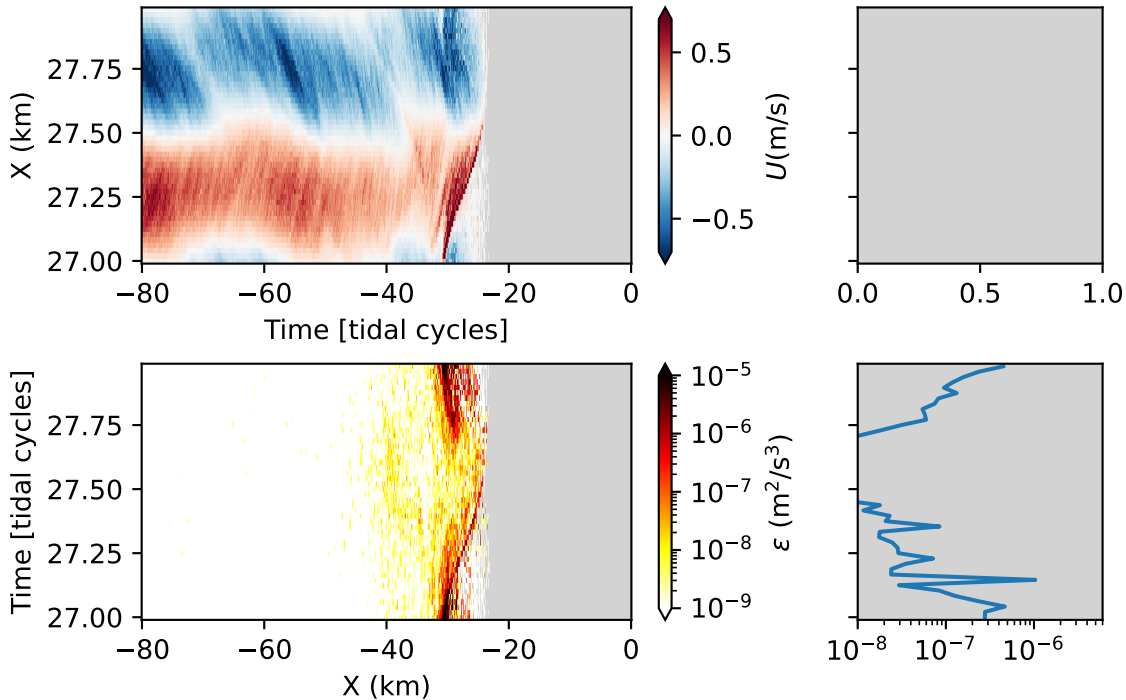
Slope2D103: Hovmoller along [25.6] isopycnal
