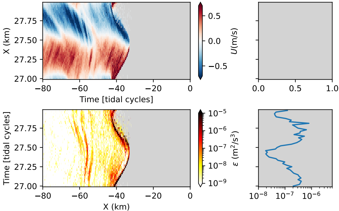
Slope2D104: Hovmoller along [25.6] isopycnal
