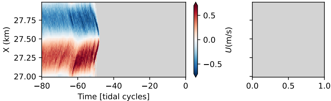
Slope2D105: Hovmoller along [25.6] isopycnal
