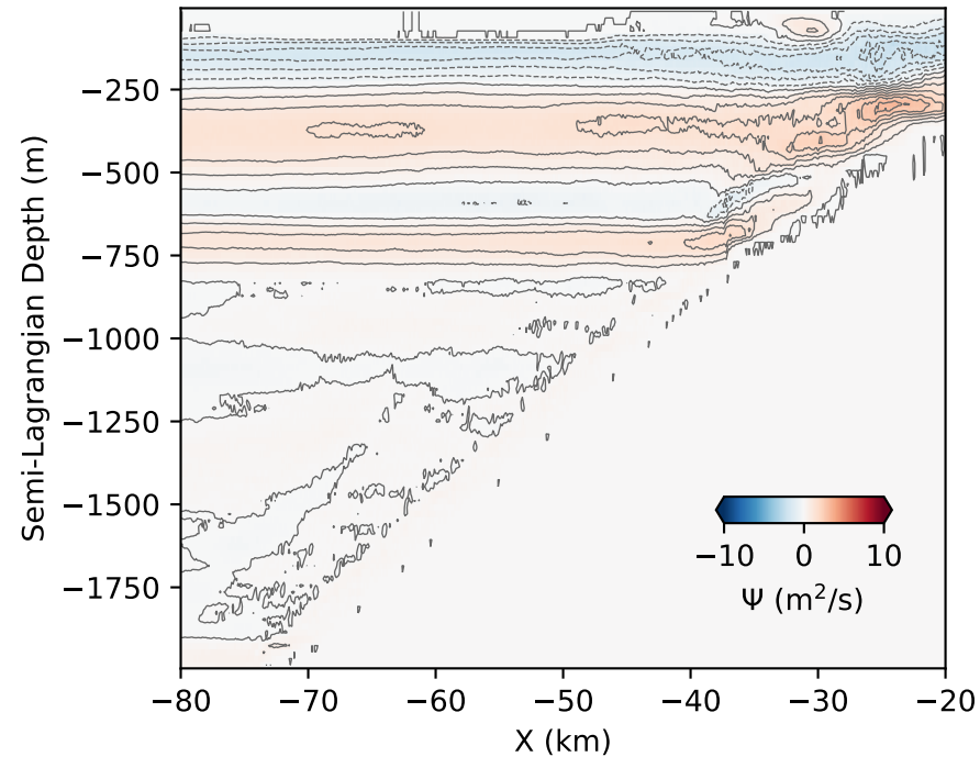
a) sub-critical slope; u_0=0.45 m/s
