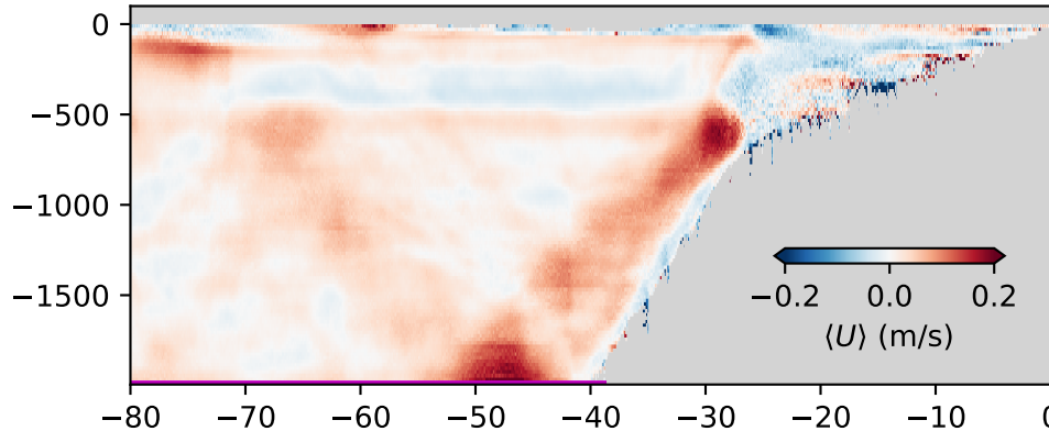
a) super-critical slope; u_0=0.45 m/s
