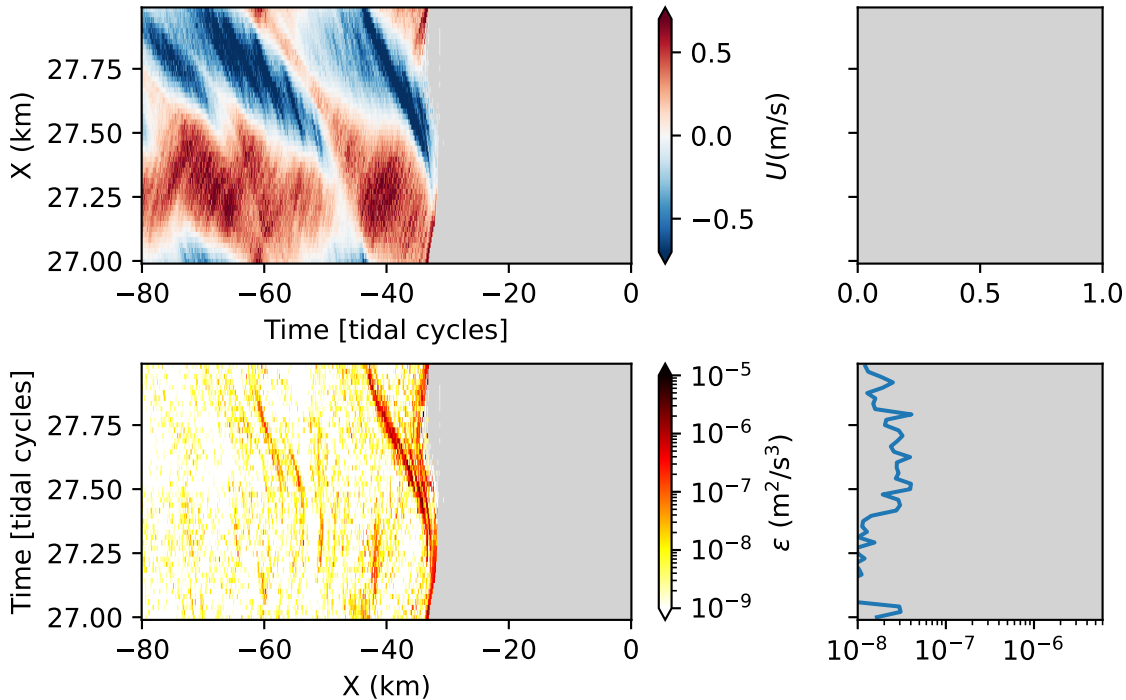
Slope2D106: Hovmoller along [25.6] isopycnal
