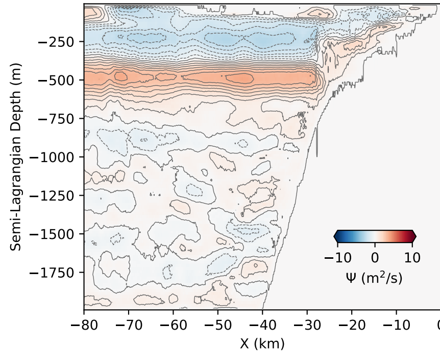
a) super-critical slope; u_0=0.45 m/s
