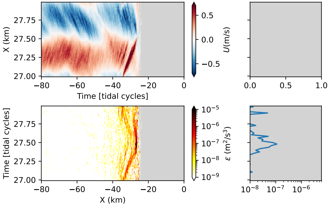
Slope2D107: Hovmoller along [25.6] isopycnal
