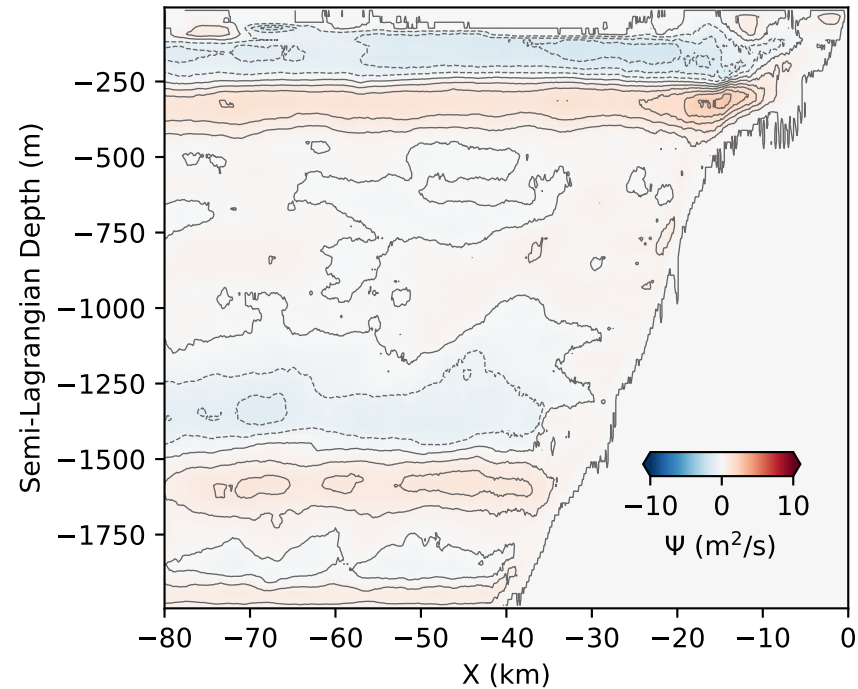
a) Multiple slopes B; u_0=0.45 m/s
