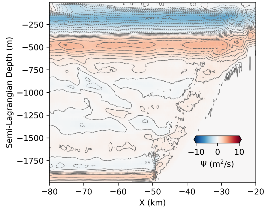
a) near-critical slope; u_0=0.45 m/s
