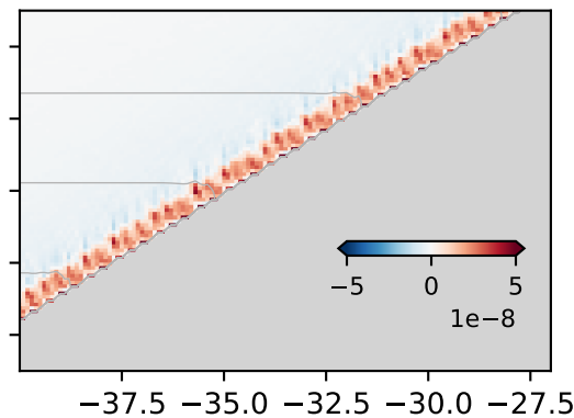
e) \langle D_t b \rangle [ \text{m/s}^3 ]
