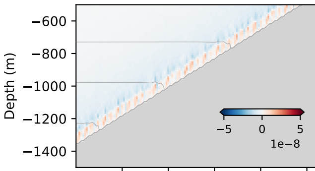
d) \langle w \rangle \langle \partial_z b \rangle [ \text{m/s}^3 ]
