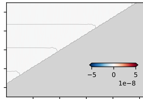
f) \partial_z \langle J_V \rangle [ \text{m/s}^3 ]
