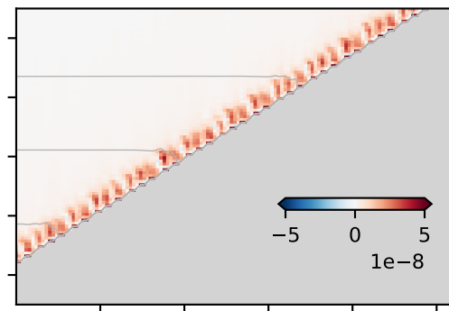
e) \langle D_t b \rangle [ \text{m/s}^3 ]
