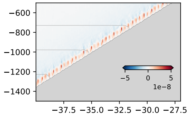
d) \langle w \rangle \langle \partial_z b \rangle [ \text{m/s}^3 ]
