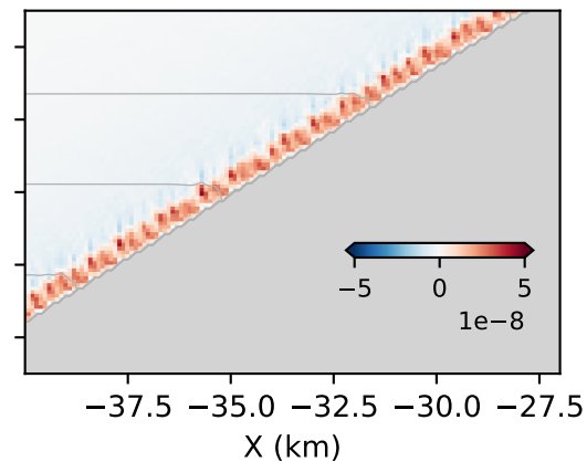
f) \partial_z \langle J_V \rangle [ \text{m/s}^3 ]
