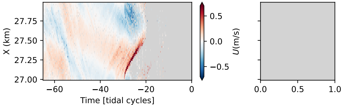
Slope2D301: Hovmoller along [25.6] isopycnal
