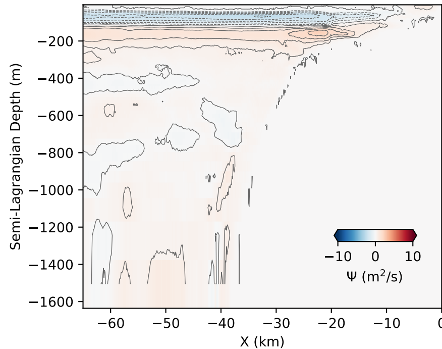
a) Exponential stratification; u_0=0.2 m/s
