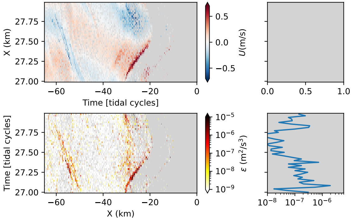
Slope2D303: Hovmoller along [25.6] isopycnal
