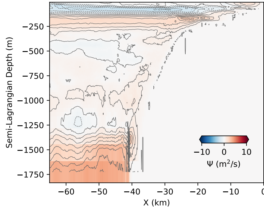
a) Exponential stratification; u_0=0.3 m/s
