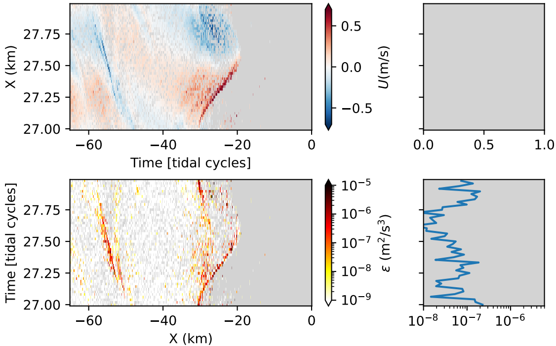
Slope2D304: Hovmoller along [25.6] isopycnal
