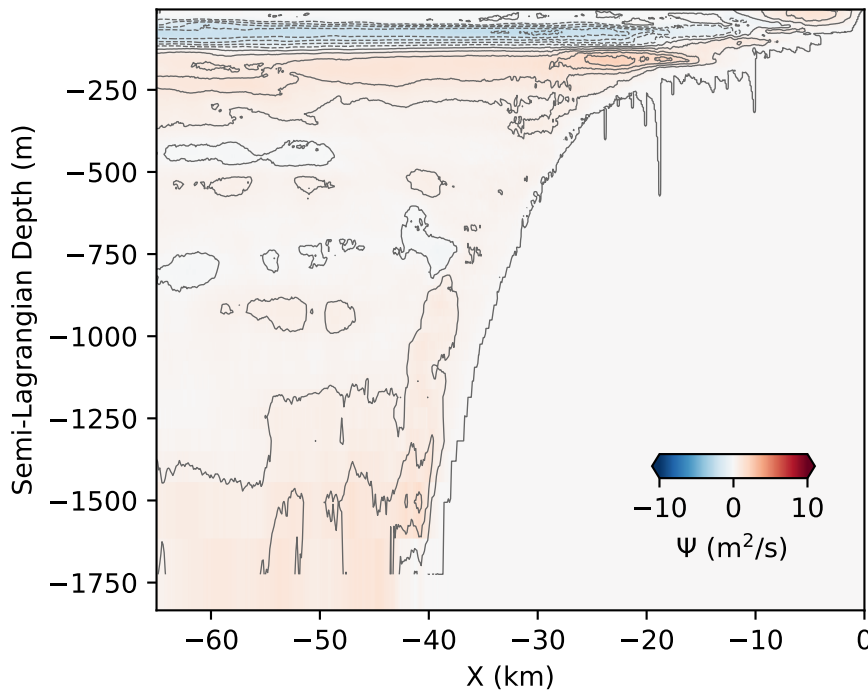
a) Exponential stratification; u_0=0.3 m/s; bottom ramp
