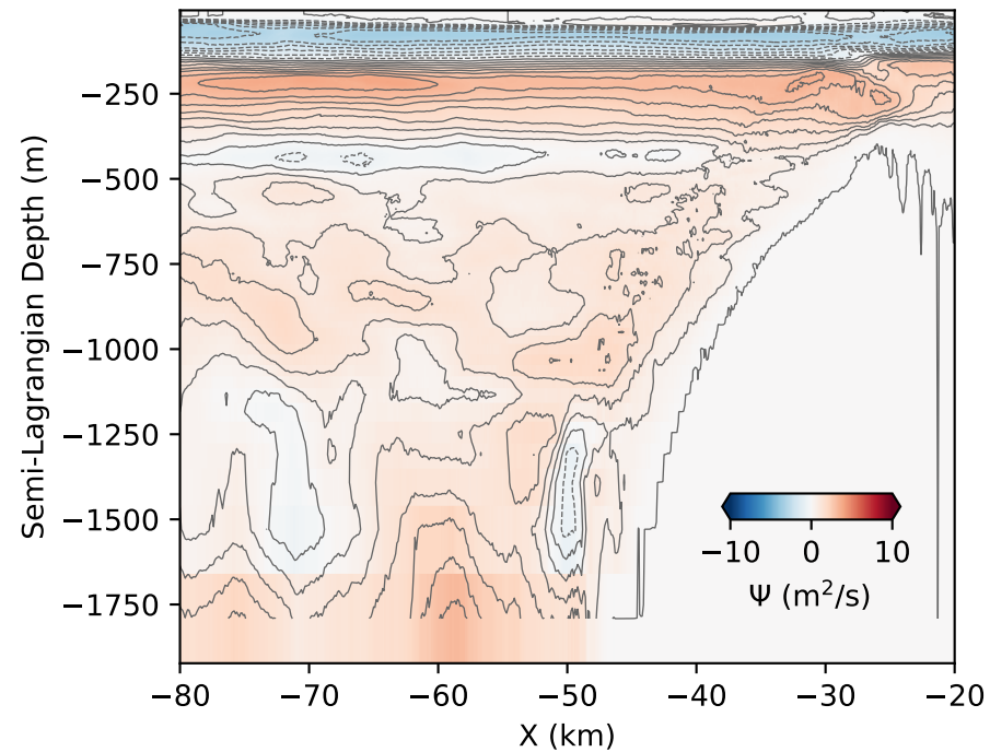
a) 3e-3 Exp; u_0=0.3 m/s; bottom ramp
