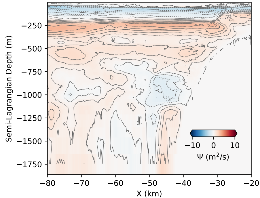
a) 3e-3 Exp; u_0=0.3 m/s; bottom ramp; subcritical 1.25
