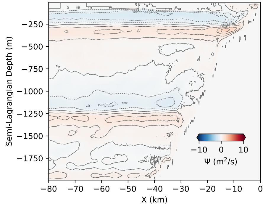
a) Multiple slopes, u_0=0.45 m/s
