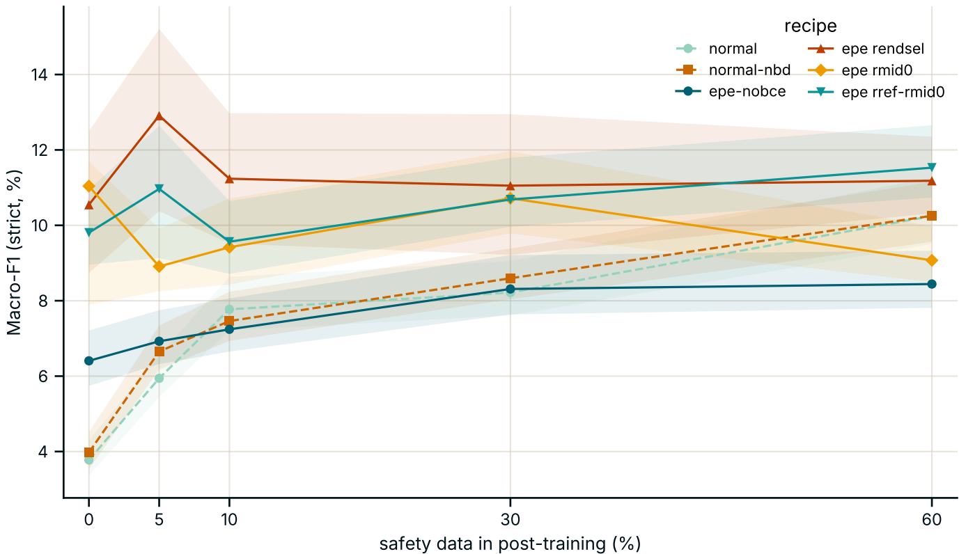
chempileedu FT, no replay + 8-shot in-context probe
