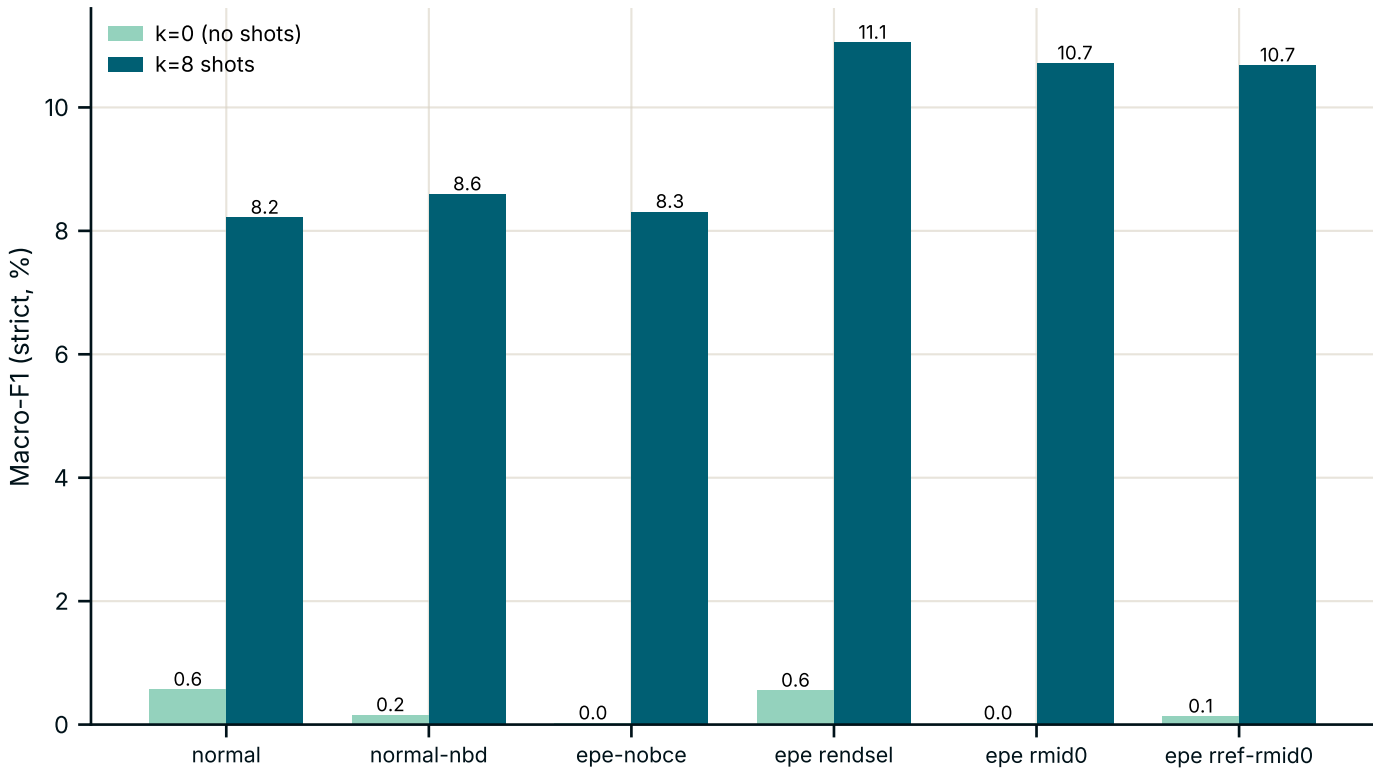
8-shot in-context probe recovers macro-F1 (s30, no replay — partial: 6 recipes, one safety point)
