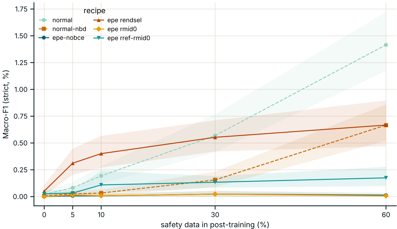
chempileedu FT, no replay — citation collapses across recipes
