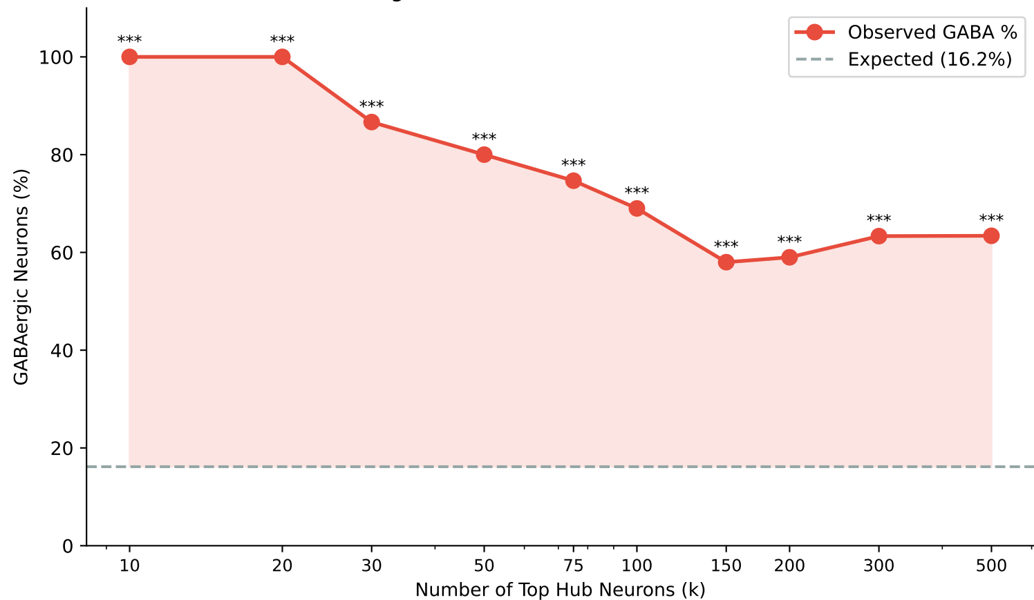
GABAergic Enrichment Across Hub Thresholds
