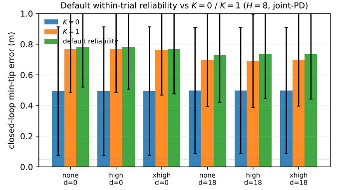
Fig. 2. Closed-loop min-tip error under the H=8 forward model and joint-PD controller for three estimators on the focused 3 noise \times 2 delay grid (mean \pm std over 10 episodes per cell). The default reliability-adaptive rule ( \beta_{0,f}=0 , \beta_{1,f}=0.5 , all fields) settles to K_f \approx 0.55 –0.72 and trails K=0 by 23–29 cm across cells; K=1 trails K=0 by 14–28 cm. The closed-loop oracle K_{cl}^* on this grid is K=0 at every cell (Appendix E); a reliability rule cannot produce K_f=0 from bounded innovation alone.
