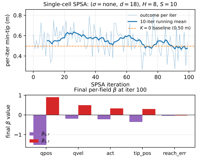
Fig. 3. Single-cell SPSA on ( \sigma=\text{none} , d=18 ) under the H=8 forward model and joint-PD controller. Top: per-iteration min-tip outcome (mean over the S=10 paired episodes per side); the dashed line marks the closed-loop K=0 baseline on this cell (0.50 m). The per-iter outcome falls from \approx 0.61 m at iteration 0 to a last-20-iter mean of \approx 0.49 m, reaching the K=0 baseline in the smoothed training-time signal; a fresh deployed evaluation of the final \beta gives 0.56 m (residual \sim 6 cm to K=0 ). Bottom: final per-field \beta vector. qpos has both the most-negative intercept ( -1.5 ) and the steepest slope ( +0.9 ); the resulting per-field correction gains K_f specialise.
