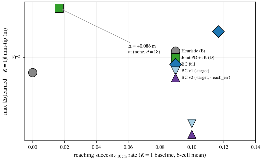
controller trade-off: reaching vs. estimator differentiation
