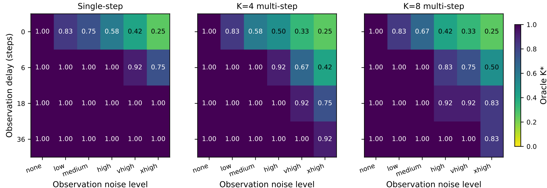
Oracle Kalman gain across the stress grid by forward-model supervision
