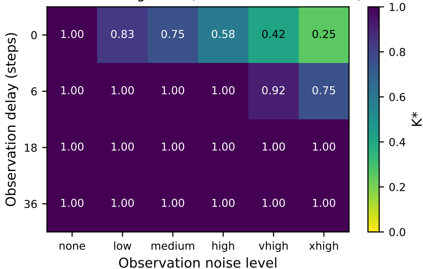
Oracle Kalman gain K^* (mean over 3 controllers)
