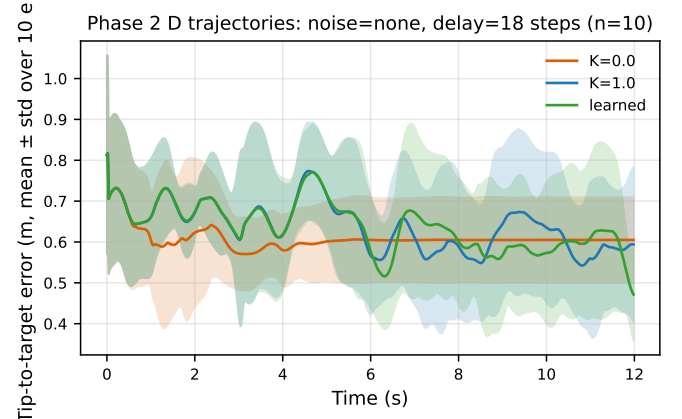
Fig. 3. Representative closed-loop trajectories at (noise=none, d=18 ): mean \pm std of min-tip error across 10 episodes for each estimator.
