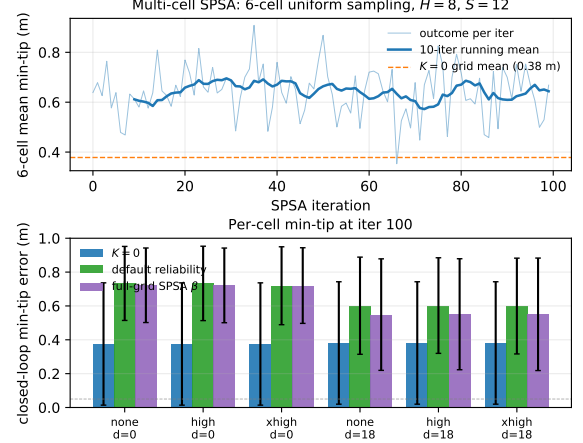
Fig. 4 Multi-cell SPSA over the focused 6-cell grid under the H=8 forward model and joint-PD controller. Top : per-iteration 6-cell-mean min-tip outcome (training-time mean over S=12 paired draws per iteration). Bottom : per-cell min-tip at deployment ( n=200 episodes per cell) for K=0 , default reliability, and the multi-cell-trained \beta . Improvement over default reliability is \approx 5 cm at delay-18 cells and \sim 0 cm at delay-0 cells; the multi-cell \beta still trails K=0 by \approx 17 cm at delay-18 cells and \approx 35 cm at delay-0 cells.
