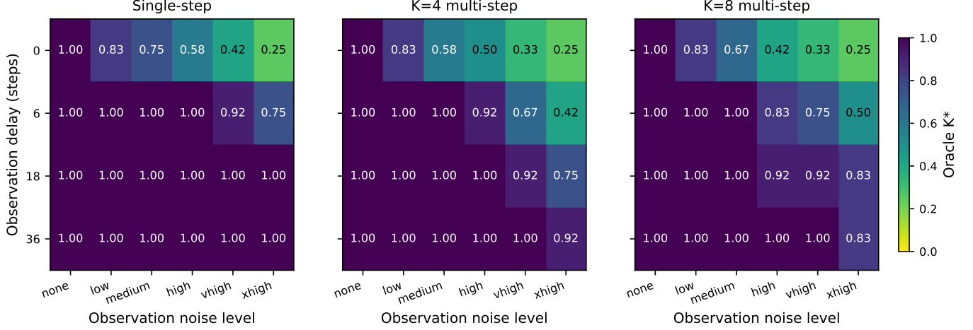
Fig. 2. Open-loop oracle Kalman gain K^* as a function of observation delay and noise level, averaged over 3 controllers and 4 delays \times 6 noise levels \times 3 controllers \times 5 K sweep = 360 cells. Three forward-model variants: single-step, K=4 multi-step, and K=8 multi-step. Under single-step supervision the K < 1 regime is confined to zero delay; multi-step supervision widens it to delay \geq 6 steps in high-noise cells.
