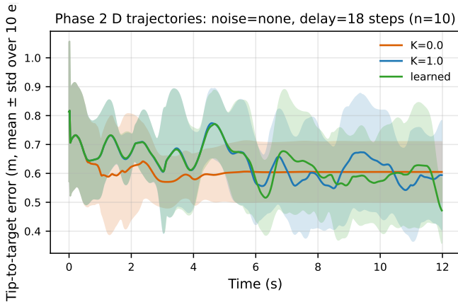
Fig. 4. Representative closed-loop trajectories at (noise=none, d=18 ): mean \pm std of min-tip error across 10 episodes for each estimator.
