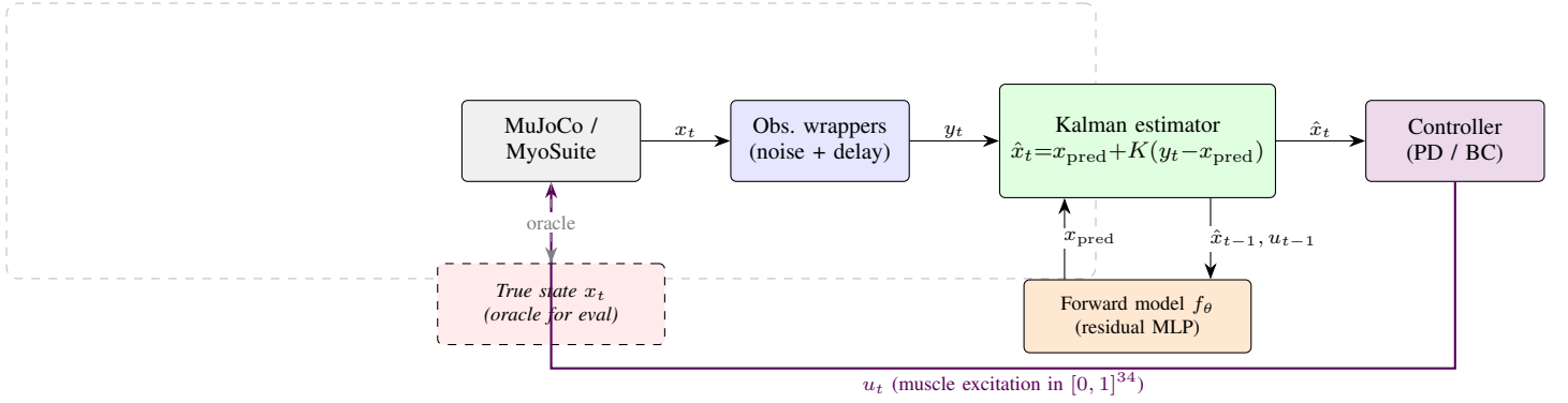
Fig. 1. Closed-loop pipeline. Each step the env’s true state x_t is filtered through observation wrappers that add per-field Gaussian noise and a fixed delay, producing y_t . The Kalman estimator combines y_t with a one-step prediction x_{\text{pred}} produced by the residual-MLP forward model f_\theta(\hat{x}_{t-1}, u_{t-1}) , weighted by a scalar gain K . The controller consumes only the estimator output \hat{x}_t and emits the next muscle excitation u_t . The true state is exposed only to the offline evaluator (dashed red box); the closed loop never accesses it.
