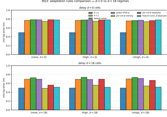
Fig. 7 Closed-loop min-tip across seven estimators on the focused 6-cell grid, faceted by delay. Top row (delay-0): all six non- K=0 rules cluster at 0.74–0.78 m; the parameterisation ceiling is shared. Bottom row (delay-18): feature-conditioned \beta deployed (cyan) reaches 0.51 m across cells — within 1.7 cm of the K=0 baseline — beating both global SPSA \beta (0.69 m) and per-cell \beta deployed (0.64 m). The delay-18 aggregation ceiling is effectively removed; the delay-0 parameterisation ceiling persists.
