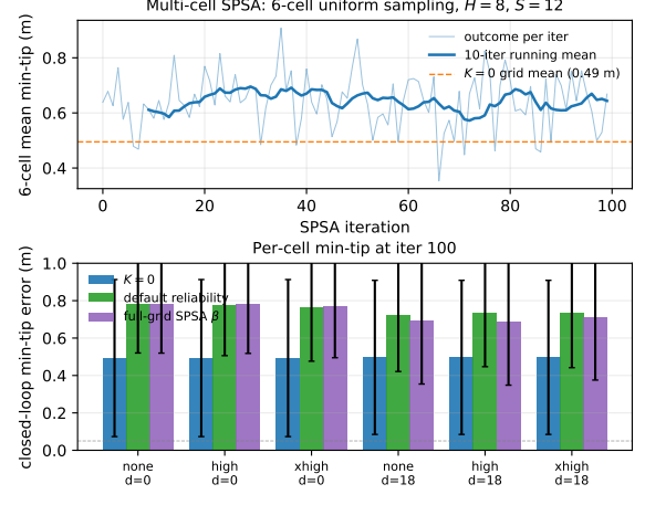
Fig. 4 Multi-cell SPSA over the focused 6-cell grid under the H=8 forward model and joint-PD controller. Top : per-iteration 6-cell-mean min-tip outcome (mean over S=12 paired draws). Bottom : per-cell min-tip at iteration 100 for K=0 , default-reliability, and the multi-cell-trained \beta . Improvement over default reliability is 3–5 cm at delay-18 cells and \sim 0 cm at delay-0 cells; the multi-cell \beta still trails K=0 by 19–22 cm at delay-18 cells.
