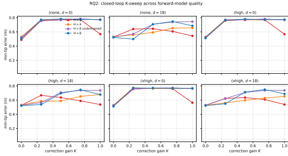
Fig. 6 Per-cell min-tip vs. K \in \{0, 0.25, 0.5, 0.75, 1\} for four forward-model conditions on the focused 6-cell grid (mean over 10 episodes per (model, cell, K )). H=8 (best) puts K_{cl}^*=0 at every cell. H=1 (worst) leaves K=0 and K=1 competitive at the three delay-18 cells; the K_{cl}^* regime begins to shift. Undertrained H=8 and H=4 are intermediate.
