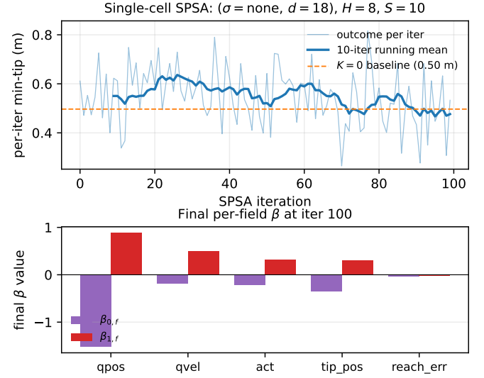
Fig. 3. Single-cell SPSA on ( \sigma=\text{none} , d=18 ) under the H=8 forward model and joint-PD controller. Top : per-iteration min-tip outcome (mean over the S=10 paired episodes per side); the dashed line marks the closed-loop K=0 baseline on this cell ( 0.50 \text{ m} ). The per-iter outcome falls from \approx 0.61 \text{ m} at iteration 0 to a last-20-iter mean of \approx 0.49 \text{ m} , reaching the K=0 baseline in the smoothed training-time signal; a fresh deployed evaluation of the final \beta gives 0.56 \text{ m} (residual \sim 6 \text{ cm} to K=0 ). Bottom : final per-field \beta vector. qpos has both the most-negative intercept ( -1.5 ) and the steepest slope ( +0.9 ); the resulting per-field correction gains K_f specialise.
