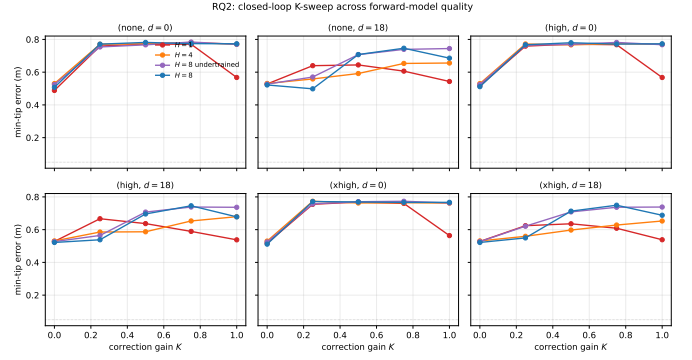
Fig. 6. Per-cell min-tip vs. K \in \{0, 0.25, 0.5, 0.75, 1\} for four forward-model conditions on the focused 6-cell grid (mean over 10 episodes per (model, cell, K )). H=8 (best) puts K_{\text{cl}}^*=0 at every cell. H=1 (worst) leaves K=0 and K=1 competitive at the three delay-18 cells; the K_{\text{cl}}^* regime begins to shift. Undertrained H=8 and H=4 are intermediate.
