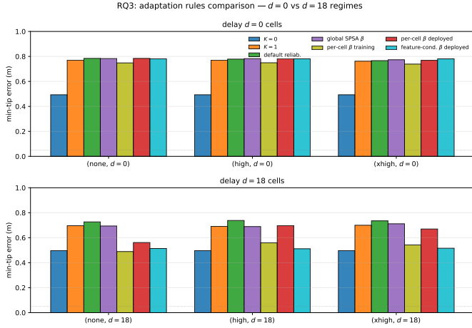
Fig. 7. Closed-loop min-tip across seven estimators on the focused 6-cell grid, faceted by delay. Top row (delay-0): all six non- K=0 rules cluster at 0.74–0.78 m; the parameterisation ceiling is shared. Bottom row (delay-18): feature-conditioned \beta deployed (cyan) reaches 0.51 m across cells — within 1.7 cm of the K=0 baseline — beating both global SPSA \beta (0.69 m) and per-cell \beta deployed (0.64 m). The context aggregation ceiling is broken.
