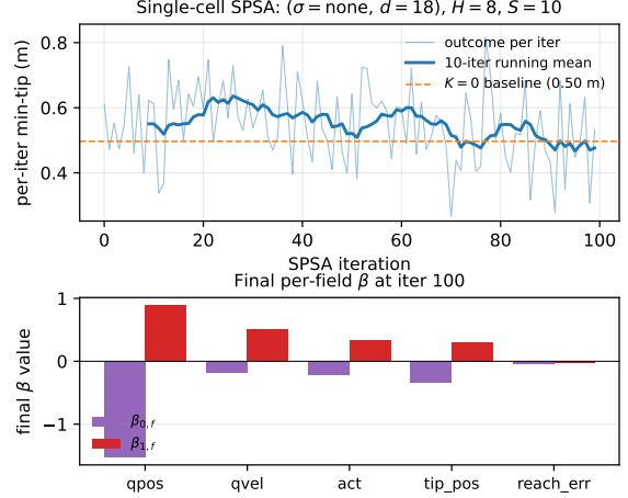
Fig. 3 Single-cell SPSA on ( \sigma=\text{none} , d=18 ) under the H=8 forward model and joint-PD controller. Top: per-iteration min-tip outcome (mean over the S=10 paired episodes per side); the dashed line marks the closed-loop K=0 baseline on this cell (0.50 m). The per-iter outcome falls from \approx 0.61 m at iteration 0 to a last-20-iter mean of \approx 0.49 m, reaching the K=0 baseline in the smoothed training-time signal; a fresh deployed evaluation of the final \beta gives 0.56 m (residual \sim 6 cm to K=0 ). Bottom: final per-field \beta vector. qpos has both the most-negative intercept ( -1.5 ) and the steepest slope ( +0.9 ); the resulting per-field correction gains K_f specialise.
