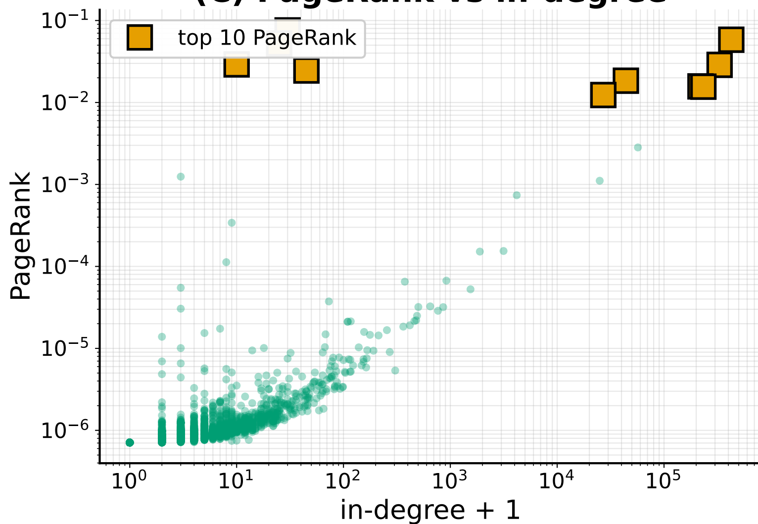
(C) PageRank vs in-degree
