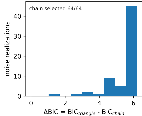
Minimum-family selection
