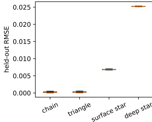
Unseen-forcing prediction
