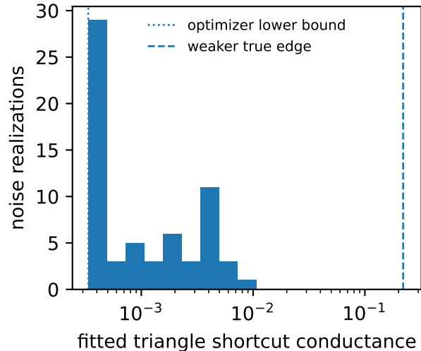
Overconnected edge shrinkage
